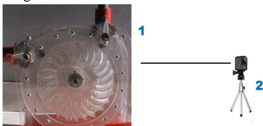
Figure 2. Experimental set-up: (1) Double nozzle cross-flow turbine, (2) Camera
