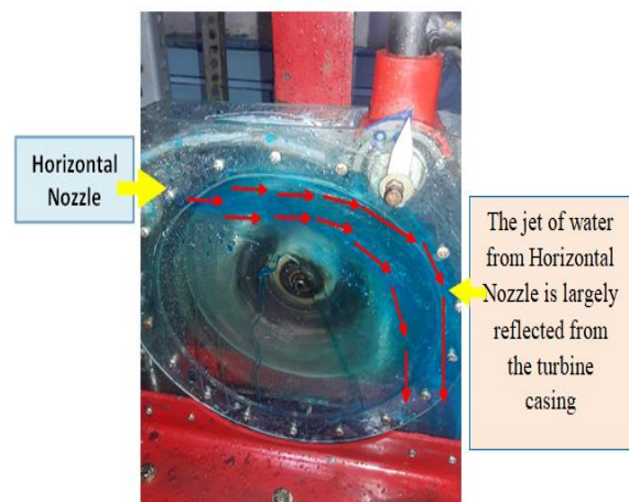
Figure 6. Fluid flow dynamics with a horizontal nozzle and nozzle vertical close
