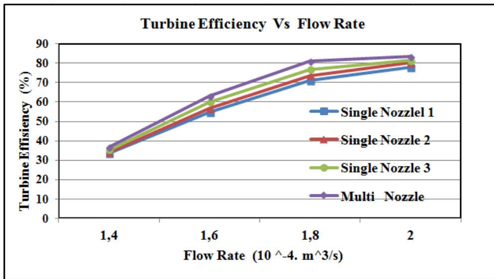
Figure-7. Turbine power graphs of water flow rate.
